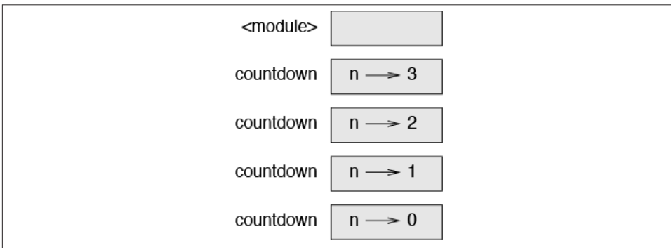
Figure 5-1. Stack diagram.
