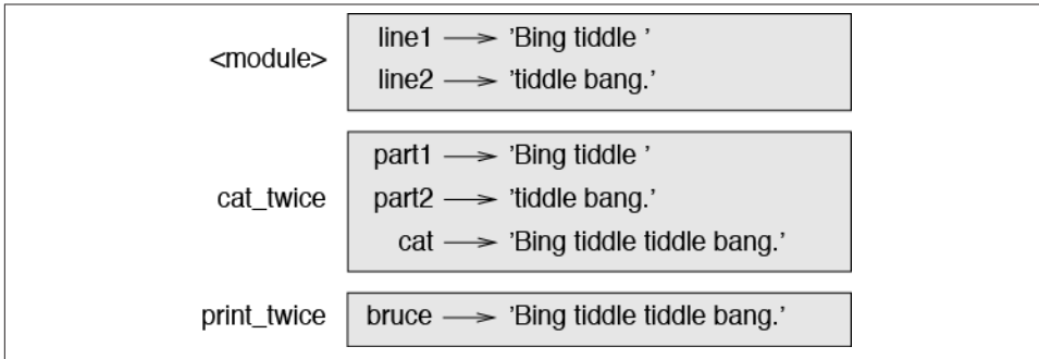
Figure 3-1. Stack diagram.
