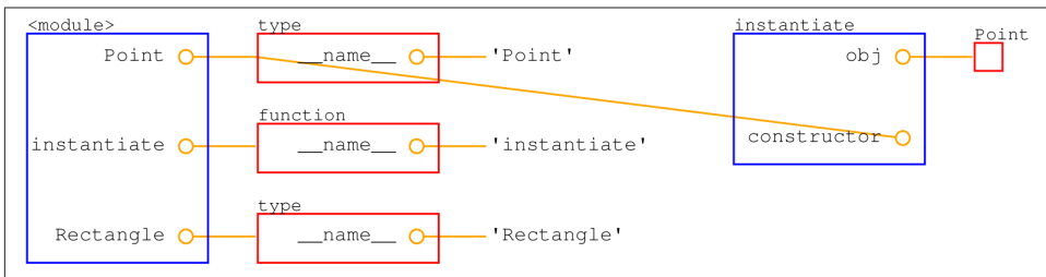
Figure C-6. Object diagram.
