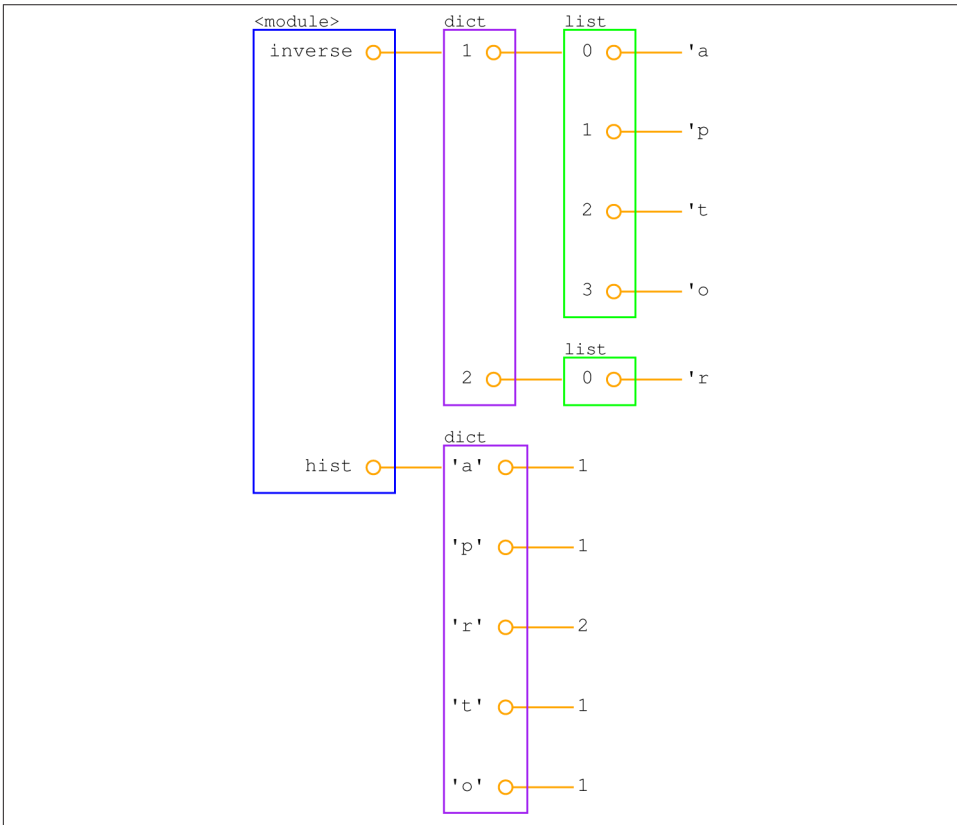
Figure C-4. Object diagram.
