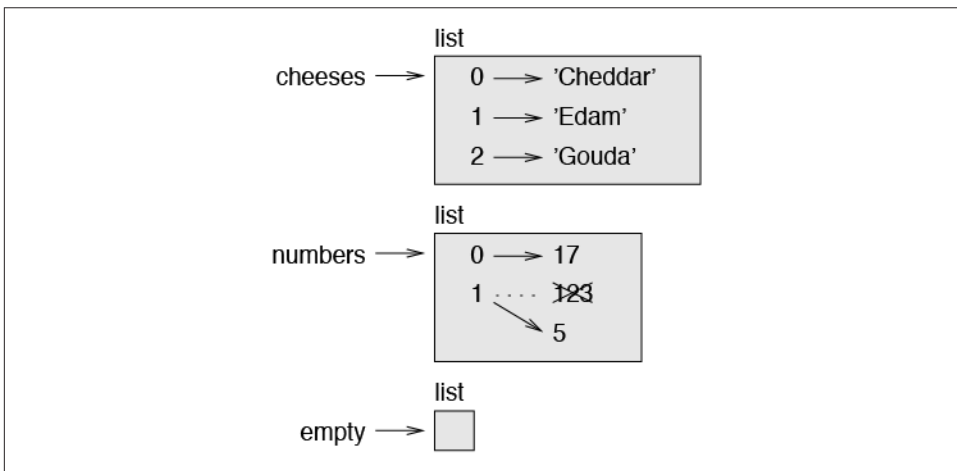
Figure 10-1. State diagram.
