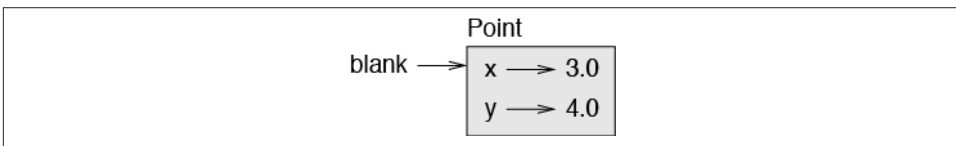
Figure 15-1. Object diagram.
